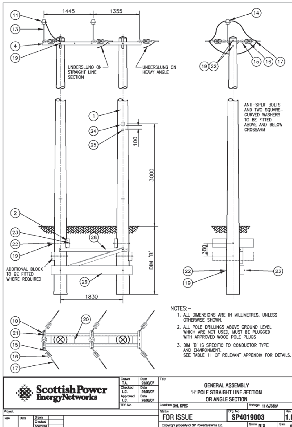
Figure 13 “H” Pole Straight Line or Angle Section (Drawing SP4019003)
